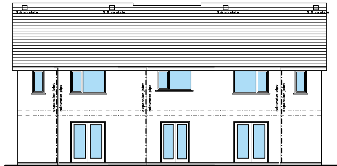
EDRYCHIAD CEFN rear elevation
