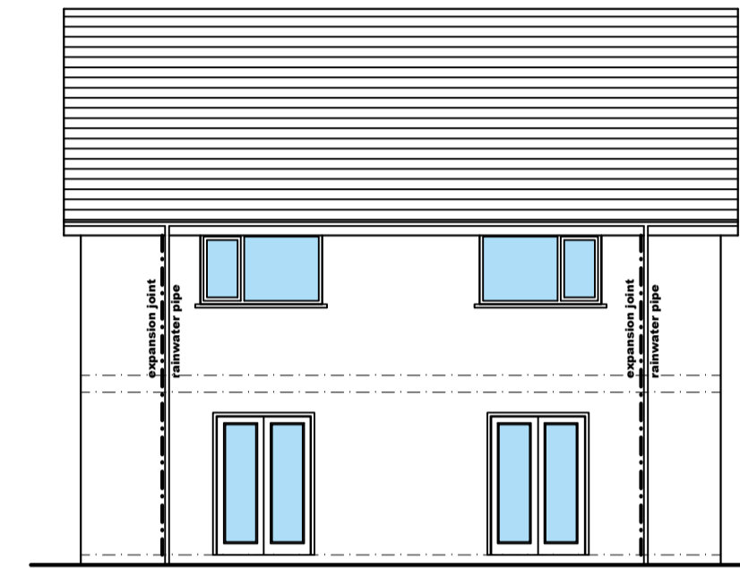
EDRYCHIAD CEFN rear elevation
