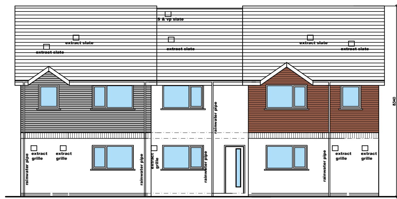
EDRYCHIAD BLAEN front elevation
