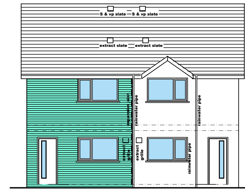
EDRYCHIAD BLAEN front elevation
